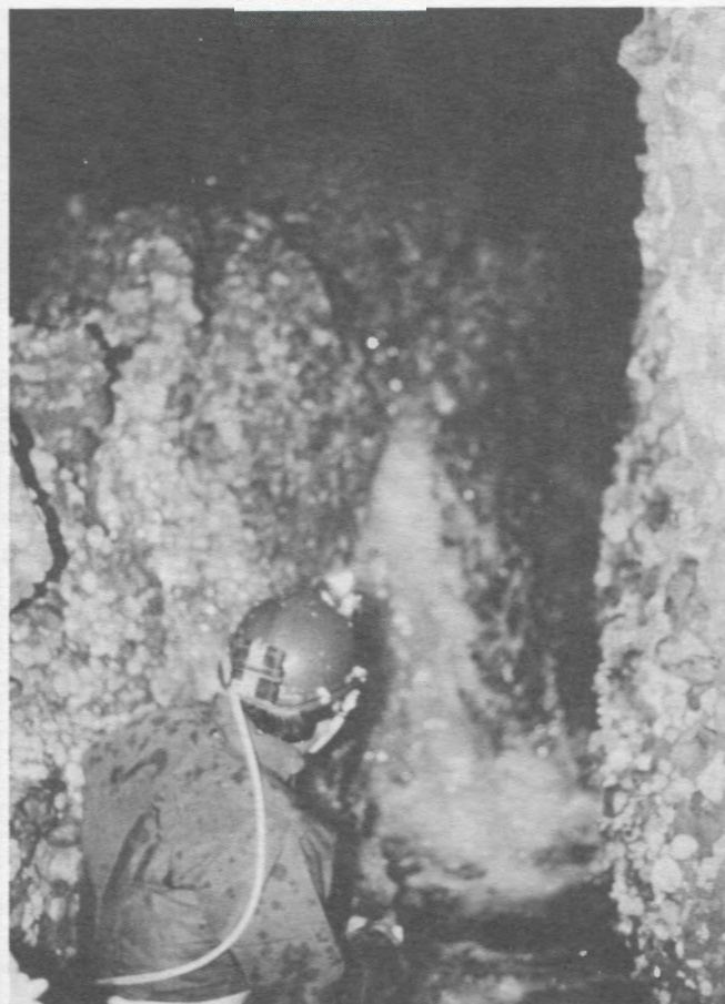
Figure 4.b.: Active underground stream in the Kuruköprü Cave. The stream existed after 2 day long heavy rainstorms around the cave. Total discharge amounts to 3m 3 /sec when the photo was taken in February 1989.
